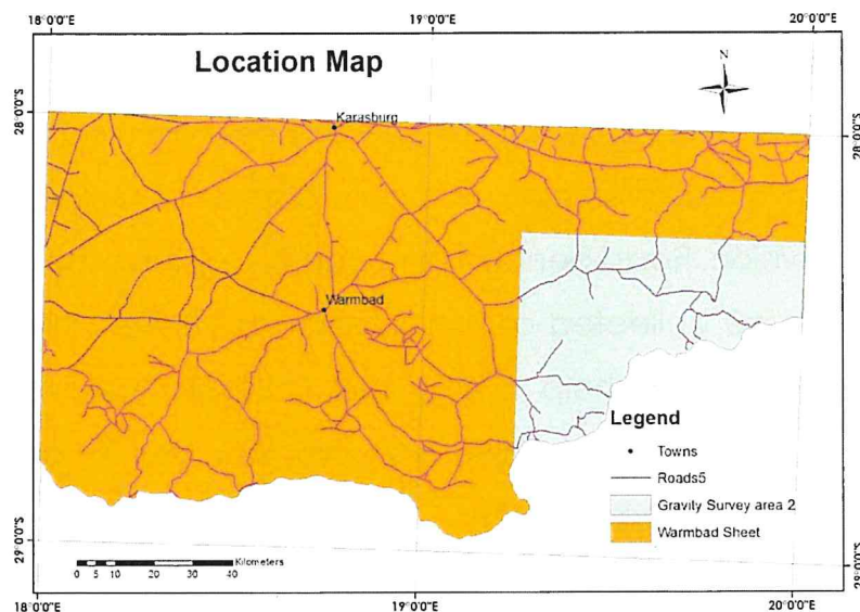
Figure 3: Geophysical survey area 2
